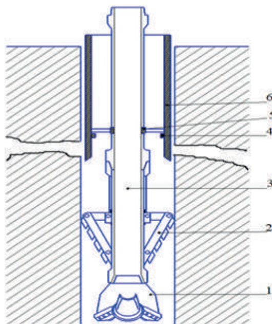
Figure 1. – Design of a drill rig for drilling with simultaneous casing of well walls. 1 – bits; 2 – expander; 3 – adapter; 4 – restrictive ring; 5 – bearing; 6 – casing pipe.
